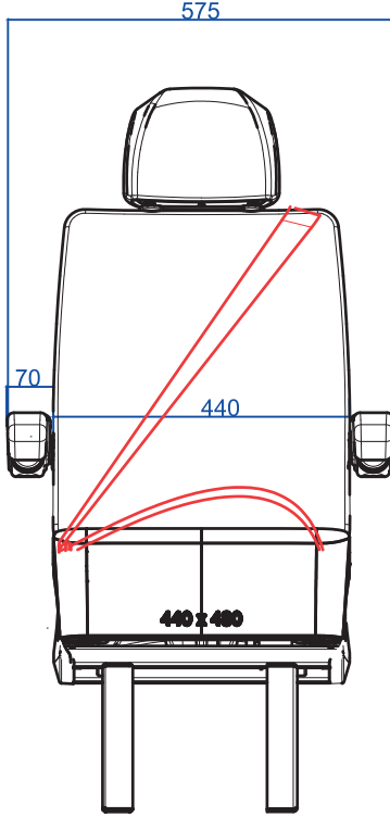
TECHNICAL DRAWING (FRONT VIEW)
